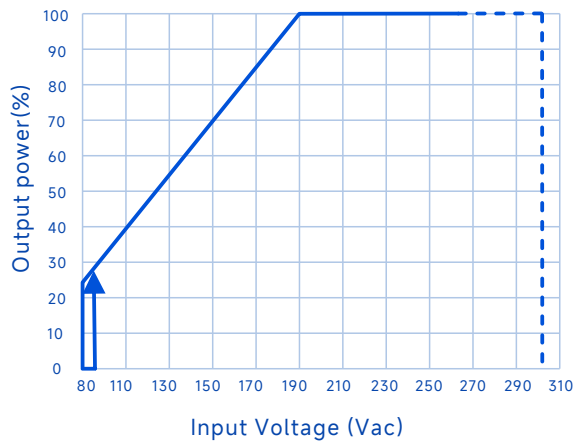
O/P Power Vs. Input Voltage (Ta Max.55°C)
